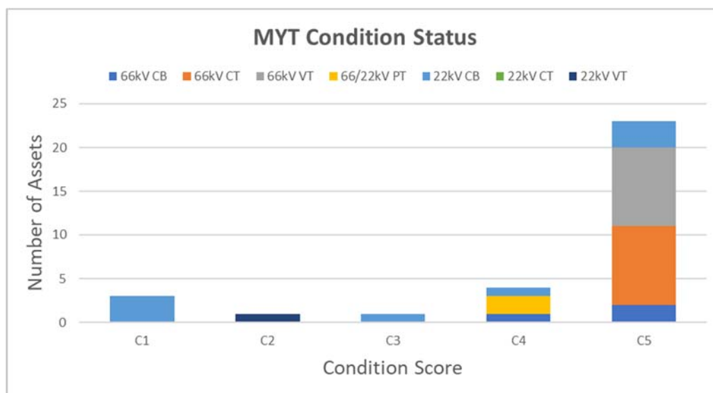
Figure 22: Number of Assets by Condition Score at MYT Zone Substation
