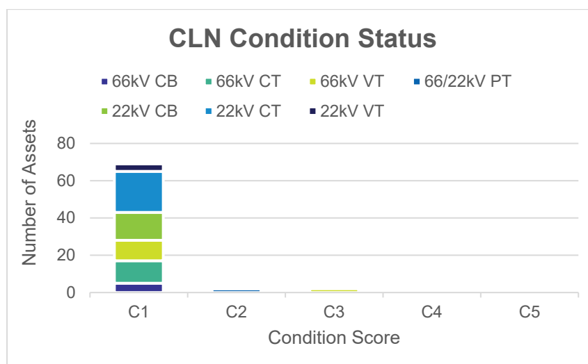
Figure 17: Number of Assets by Condition Score at CLN Zone Substation
