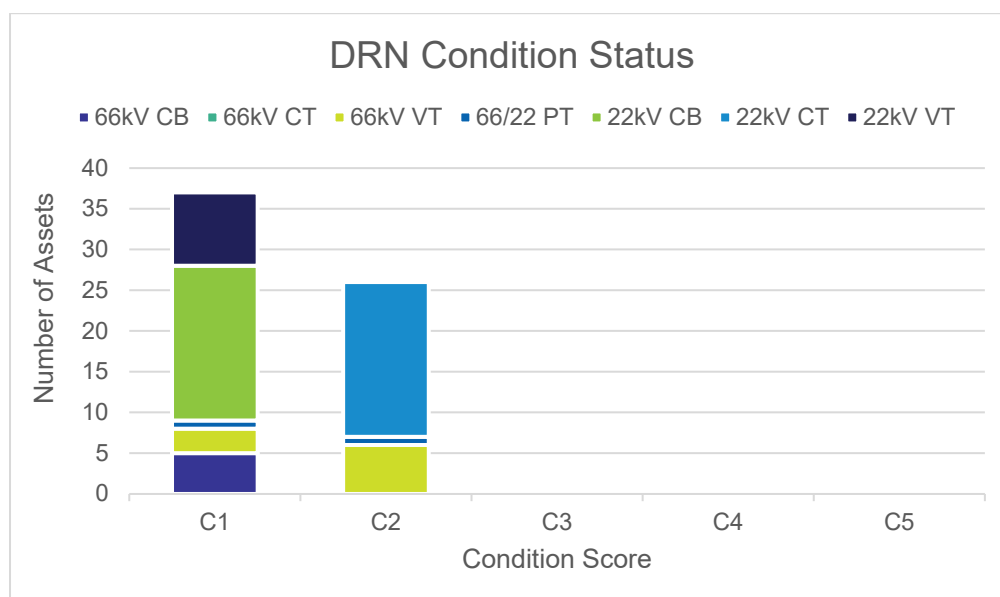
Figure 18: Number of Assets by Condition Score at DRN Zone Substation
