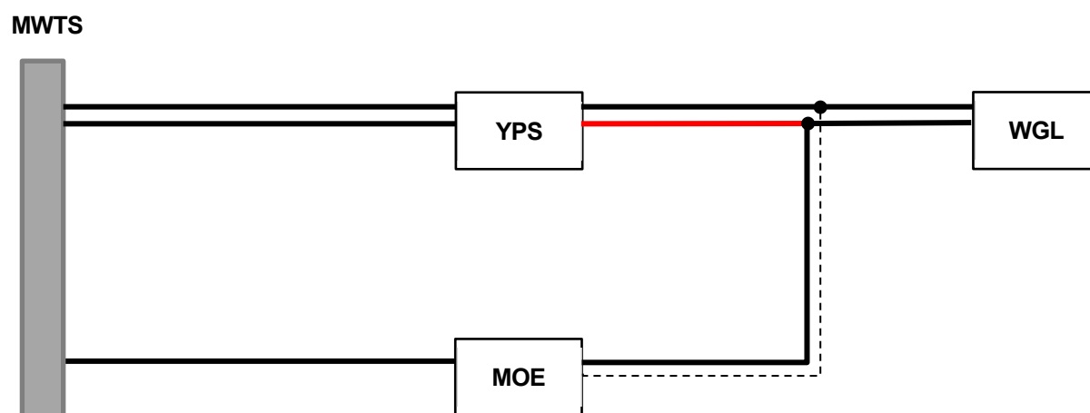
Figure 13: MWTS-YPS-MOE-WGL 66 kV Loop
