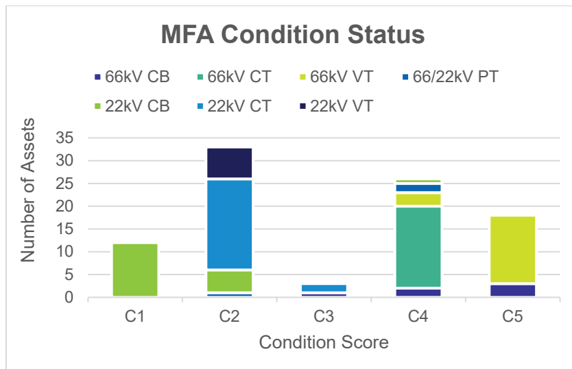
Figure 20 : Number of Assets by Condition Score at MFA Zone Substation
