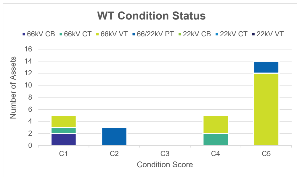
Figure 29: Number of Assets by Condition Score at WT Zone substation
