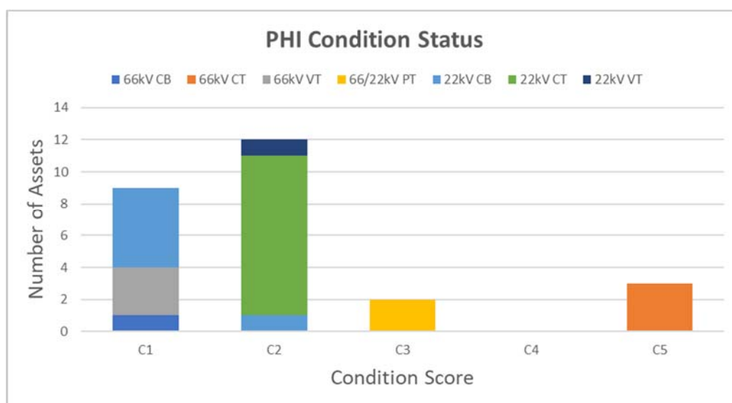
Figure 25: Number of Assets by Condition Score at PHI Zone Substation
