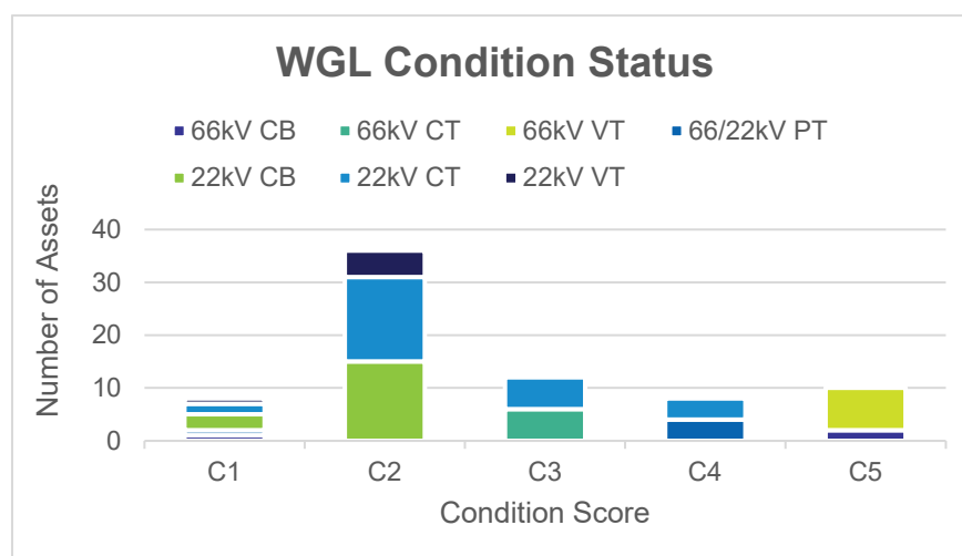
Figure 31: Number of Assets by Condition Score at WGL Zone substation
