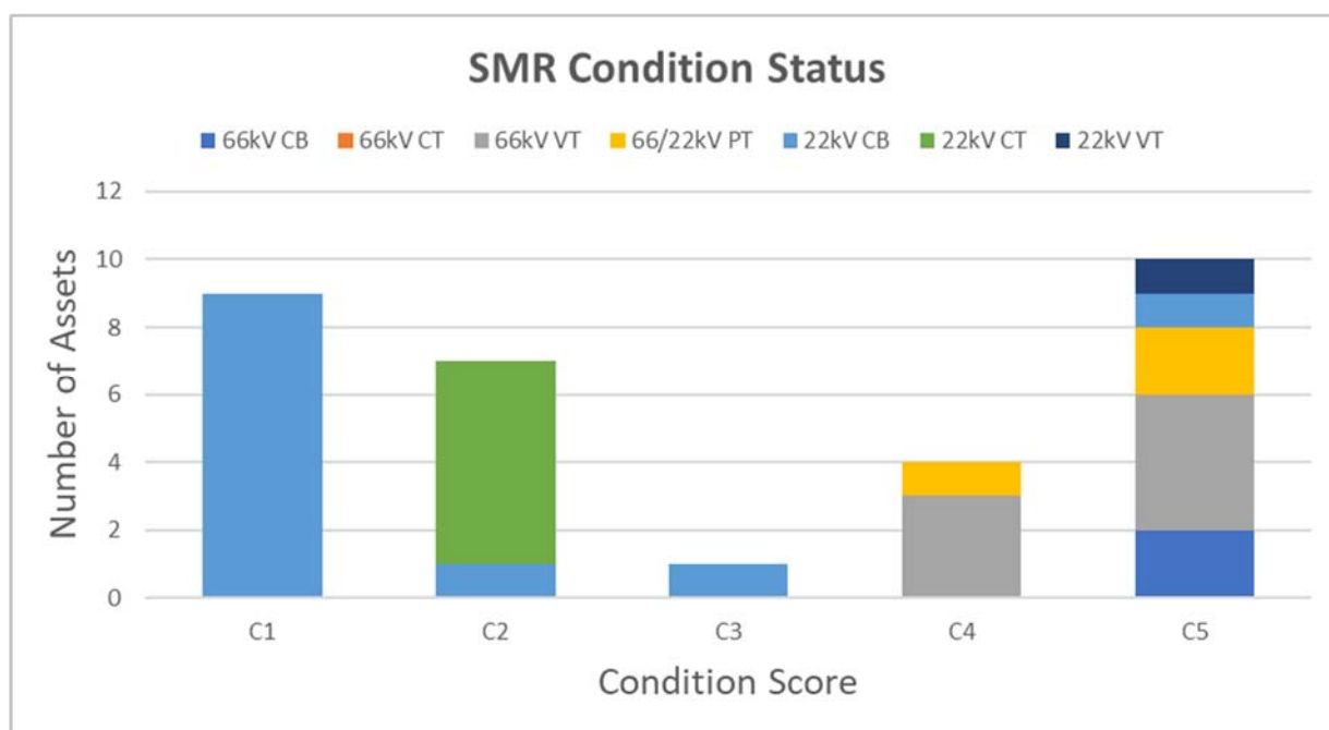
Figure 26: Number of Assets by Condition Score at SMR Zone Substation
