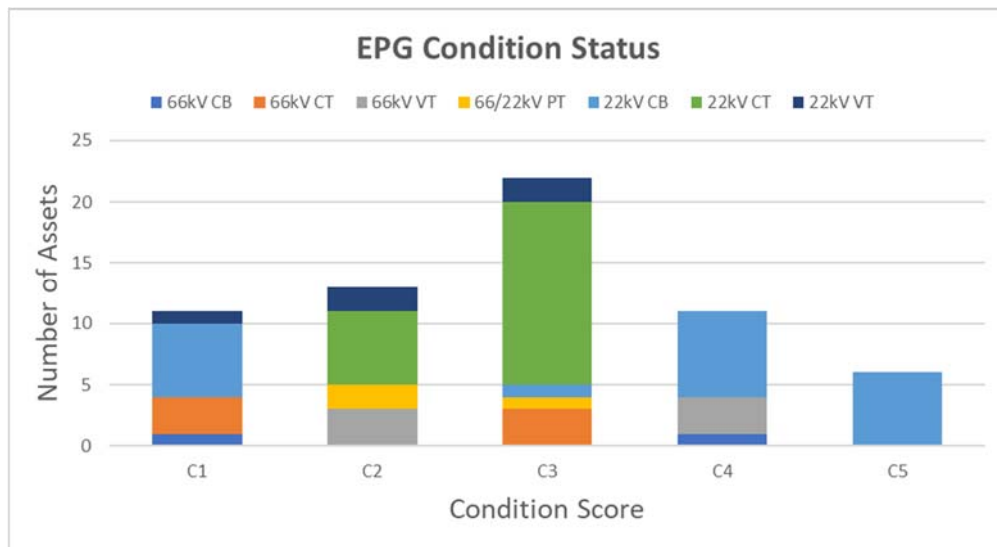
Figure 19: Number of Assets by Condition Score at EPG Zone Substation
