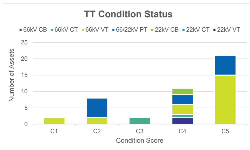
Figure 27: Number of Assets by Condition Score at risk at TT Zone substation
