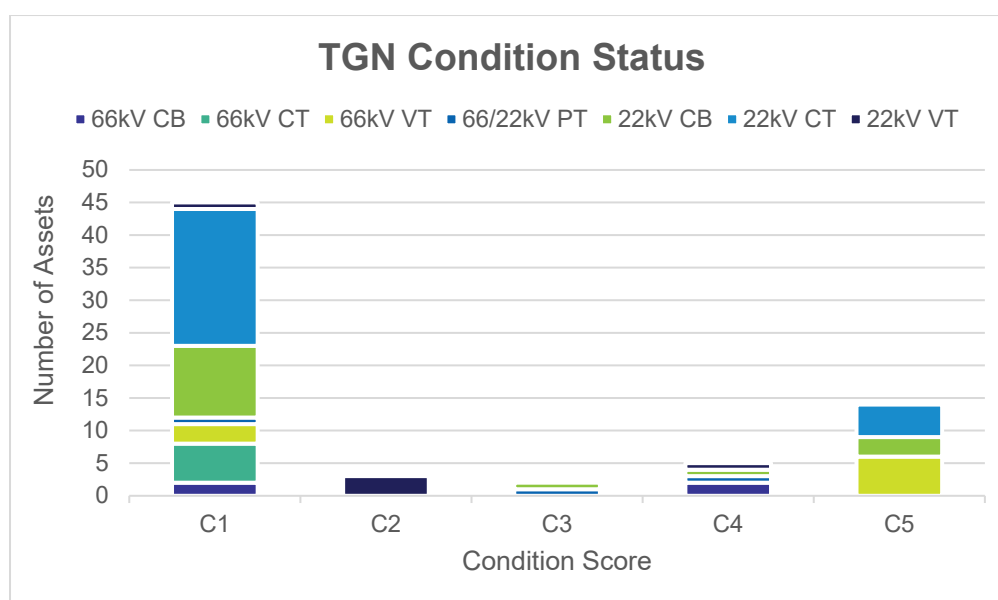
Figure 28: Number of Assets by Condition Score at TGN Zone substation
